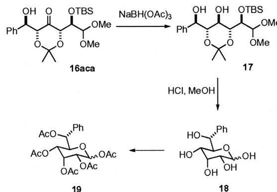
Scheme 4. Synthesis of 6-C-phenyl-D-glycero-D-allohexopyranose.
