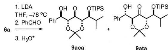
Scheme 3. The second aldol reaction via lithium enolate.
