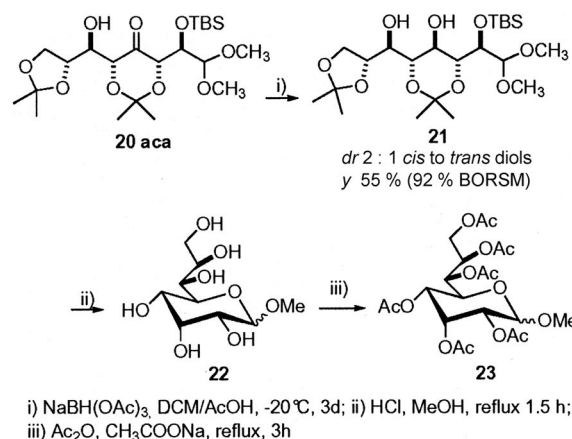
Scheme 5. Synthesis of a D-erythro-D-allopyranose derivative.
