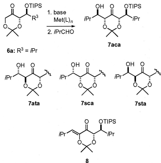
Scheme 2. The second aldol reaction.
