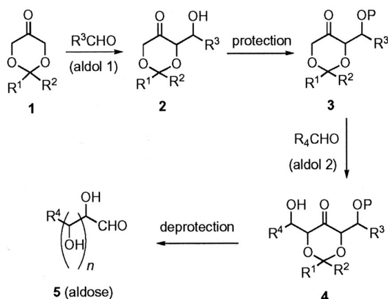
Scheme 1. Synthetic strategy towards higher aldoses.
